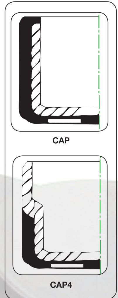
Illustration A End Cap Profiles
